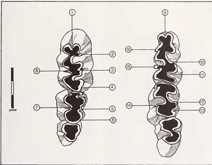
Fig. 3. Left upper molar row (A) and left lower molar row (B) of a female of A. alterus from El Infiernillo, Tucumán Province, Argentina: 1-anteromedian flexus of M1; 2-anteroloph-parastyle of M1; 3-mesostyle-mesoloph of M1; 4-posteroloph-posterostyle of M1; 5-mesostyle-mesoloph of M2; 6-posteroloph-posterostyle of M2; 7-enterostyle of M2; 8-enterostyle of M1; 9-anteromedian flexid of m1; 10-mesostylid-mesolophid of m1; 11-posterolophid-posterostylid of m1; 12-mesostylid-mesolophid of m2; 13-posterolophid-posterostylid of m2; 14-ectostylid of m2; 15-ectostylid of m1; and 16-protostylid of m1
